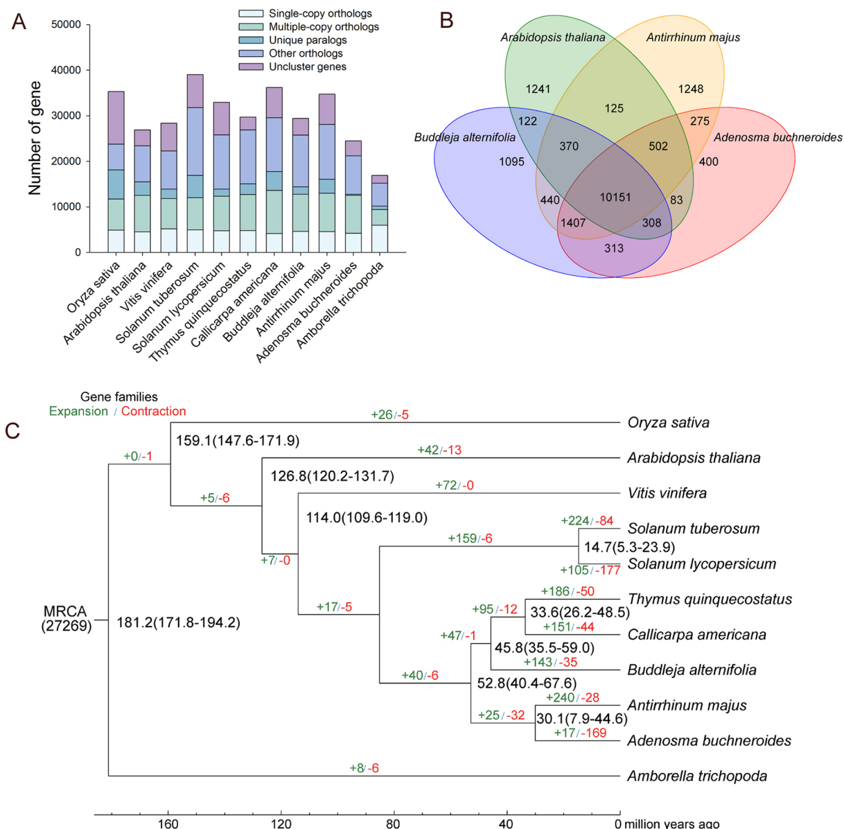
Fig. 4 Comparative genomics and phylogenetic analyses. (A) Classification and statistics of common and lineage-specific genes in A. buchneroides and other representative plant species. (B) Venn diagram of orthologous genes shared among A. buchneroides and three other species. (C) Phylogenetic analysis, gene family expansion/contraction analyses and divergence time estimations. Inferred divergence times are denoted at each node in black. Gene family expansion and contraction are indicated in green and red, respectively.
